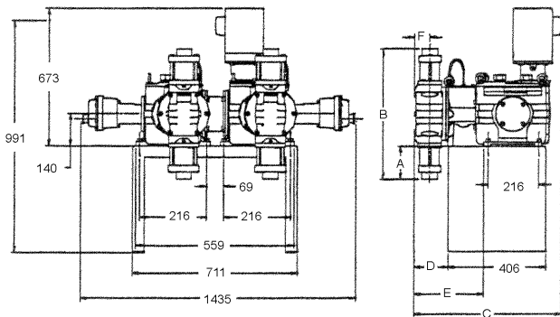
Double Simplex with Automatic Actuator
