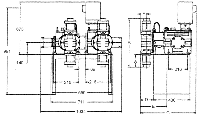
Double Simplex with Manual Stroke Control
