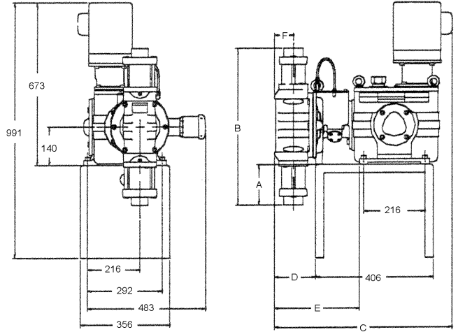
Simplex with Manual Stroke Control
