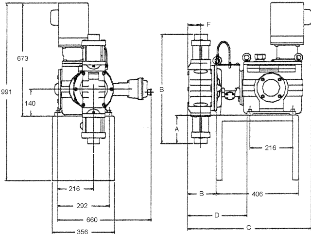
Simplex with Automatic Actuator
